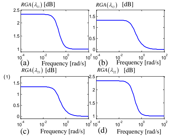
Figure 2: Relative Gain Array (RGA)
